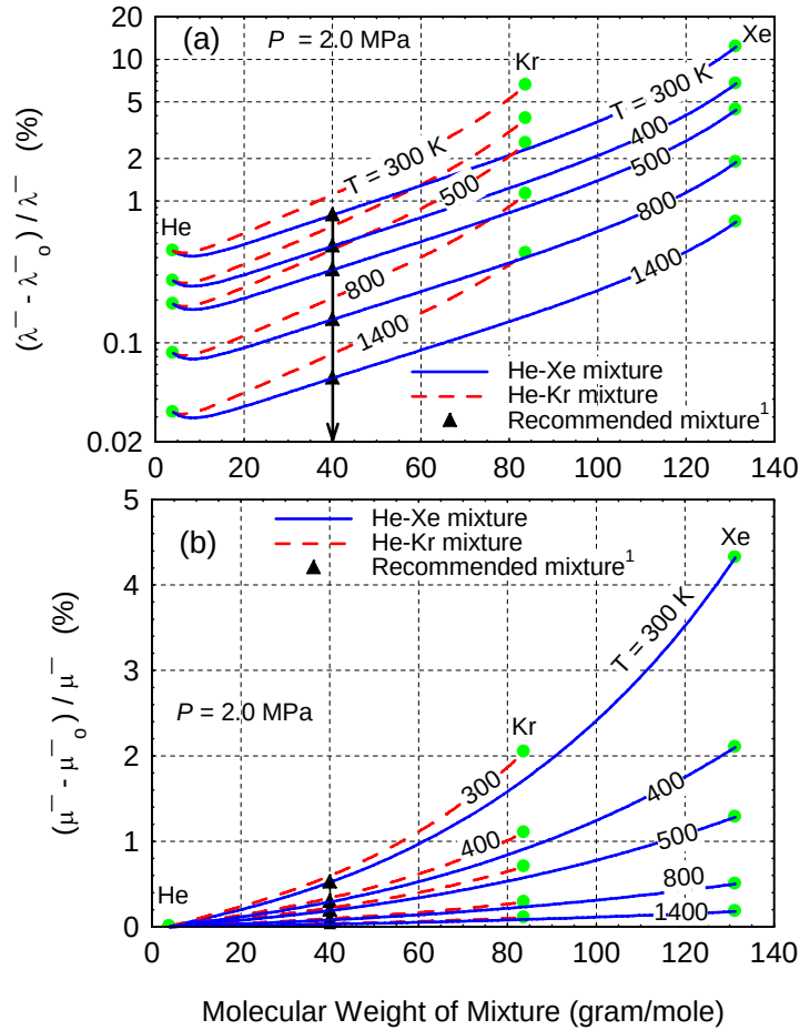
Figure 8. Dynamic viscosities and thermal conductivities of dense binary gas mixtures.
