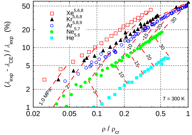
Figure 1. Thermal conductivity of dense noble gases.
