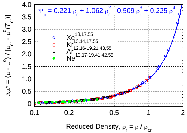
Figure 2. Reduced, excess viscosity of noble gases.
