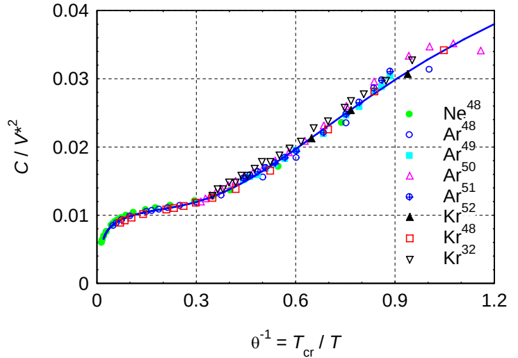
Figure 5. Reduced 3 rd virial coefficients of noble gases.
