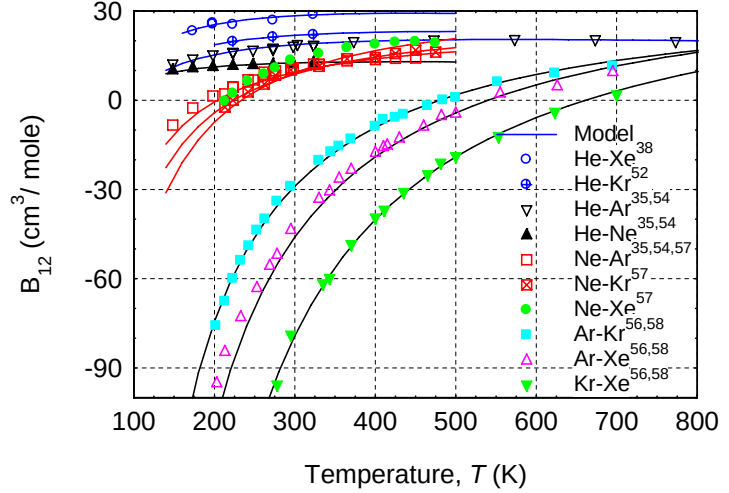
Figure 6. Second virial interaction coefficients.
