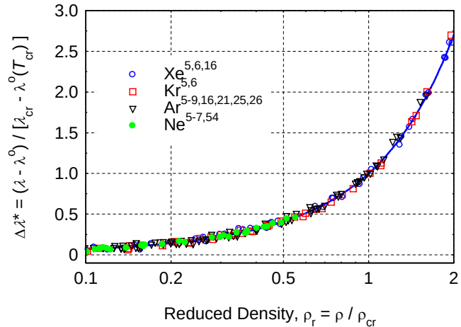
Figure 3. Reduced, excess conductivity of noble gases.
