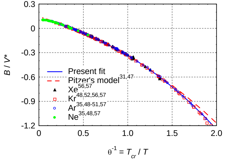
Figure 4. Reduced 2 nd virial coefficients of noble gases.
